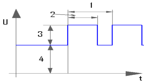
Figure 4. Components of the signal provided by the electronic control circuit
